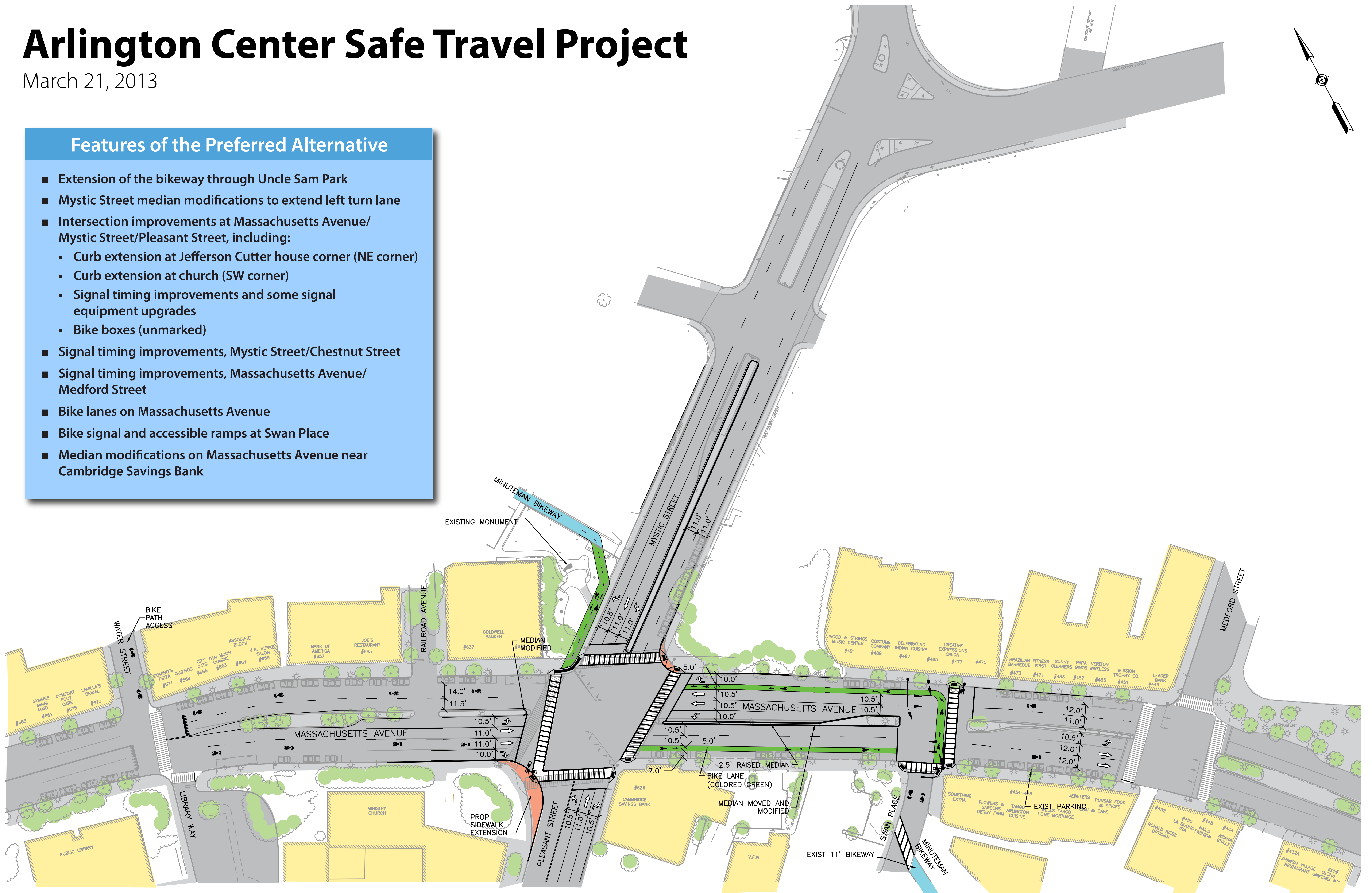
Arlington Conceptual Site Plan Addition of Bike Lanes between Water St and Swan Pl, Median Modified
