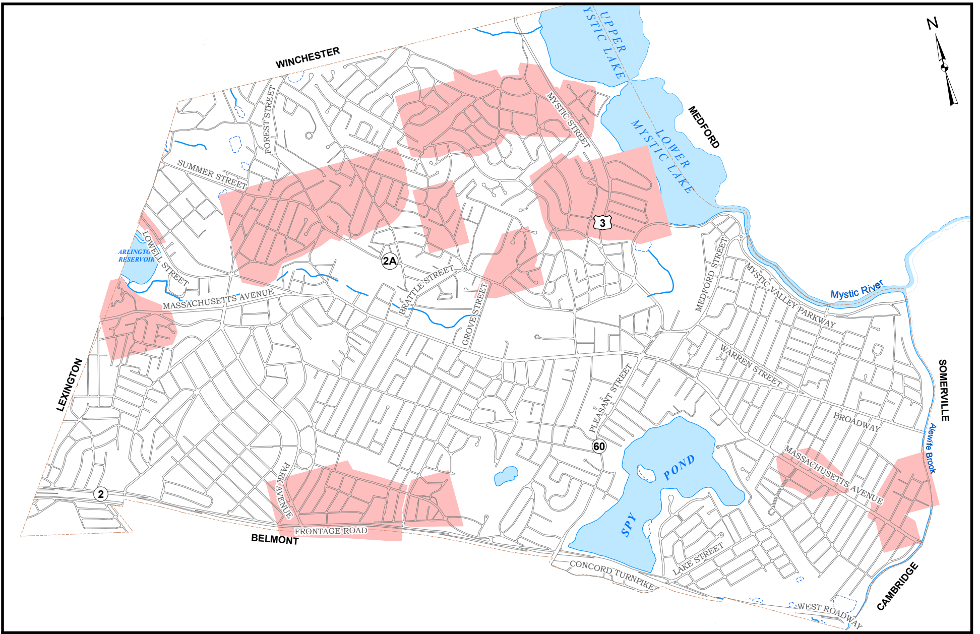
FIGURE 1 TOWN OF ARLINGTON, MASSACHUSETTS PHASE #4 SEWER REHABILITATIONS AREAS
