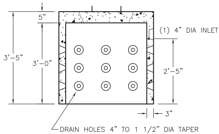
SECTION VIEW
