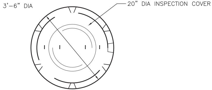
PLAN VIEW
