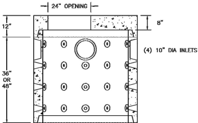
SECTION VIEW
