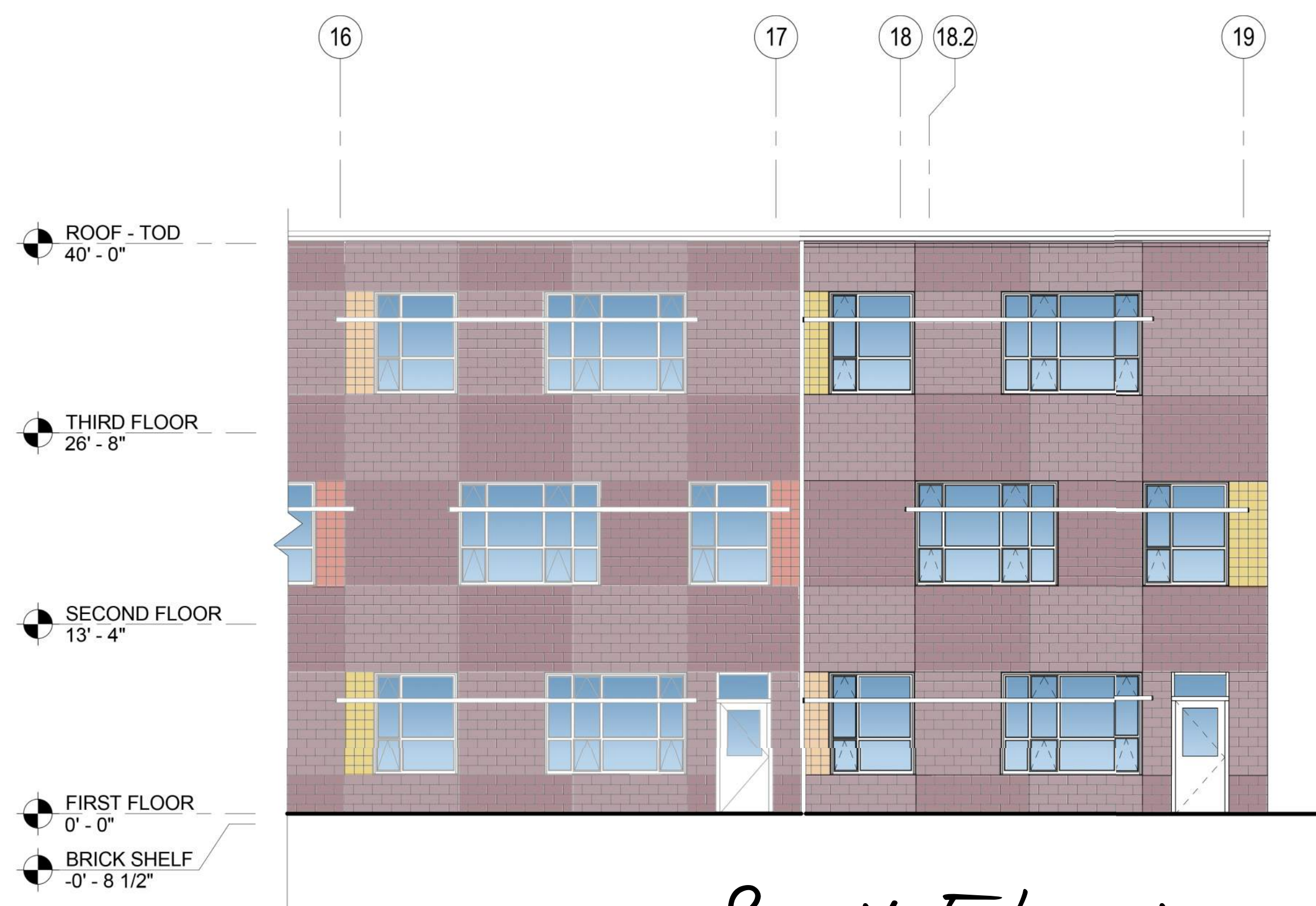
South Elevation
