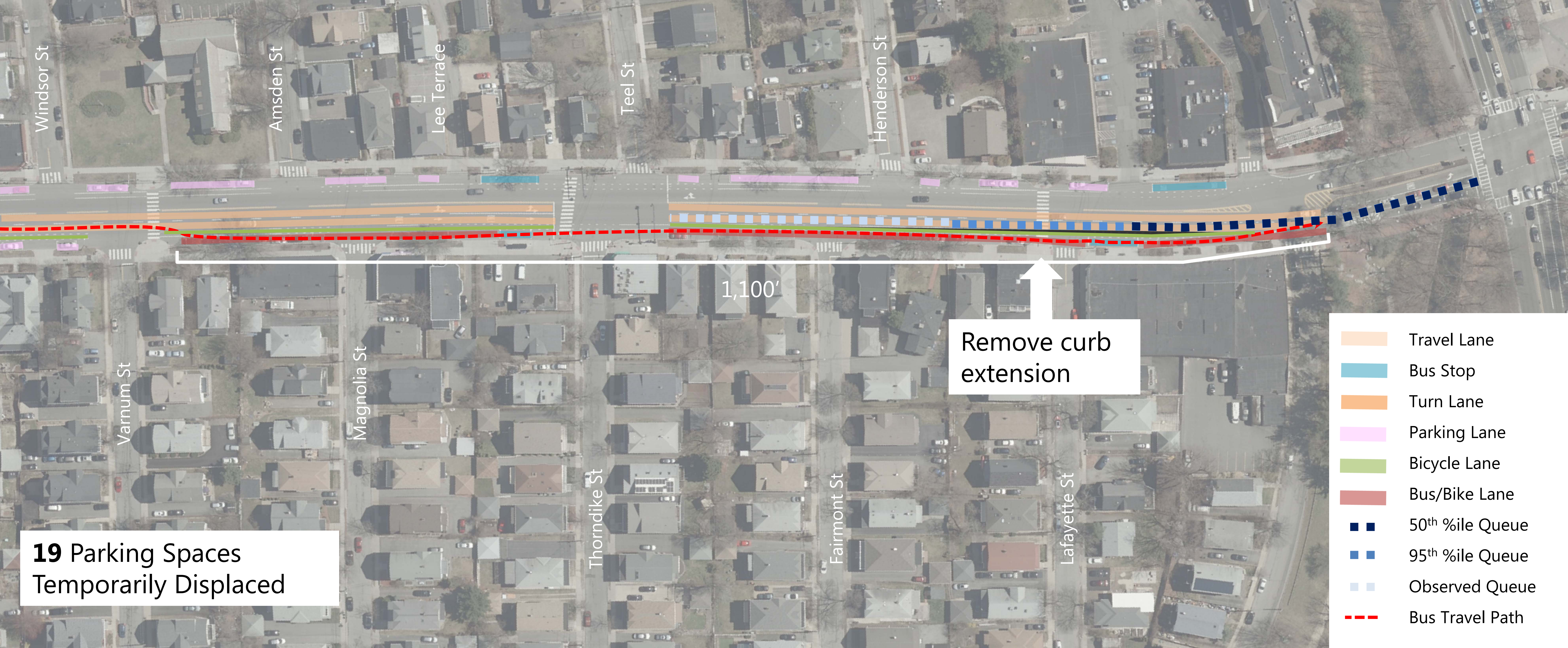
Option 2 – Provide Curbside Bus Lane from Varnum to Alewife Brook Parkway Massachusetts Avenue from Lake Street to Alewife Brook Parkway | Arlington BRT Pilot Project
