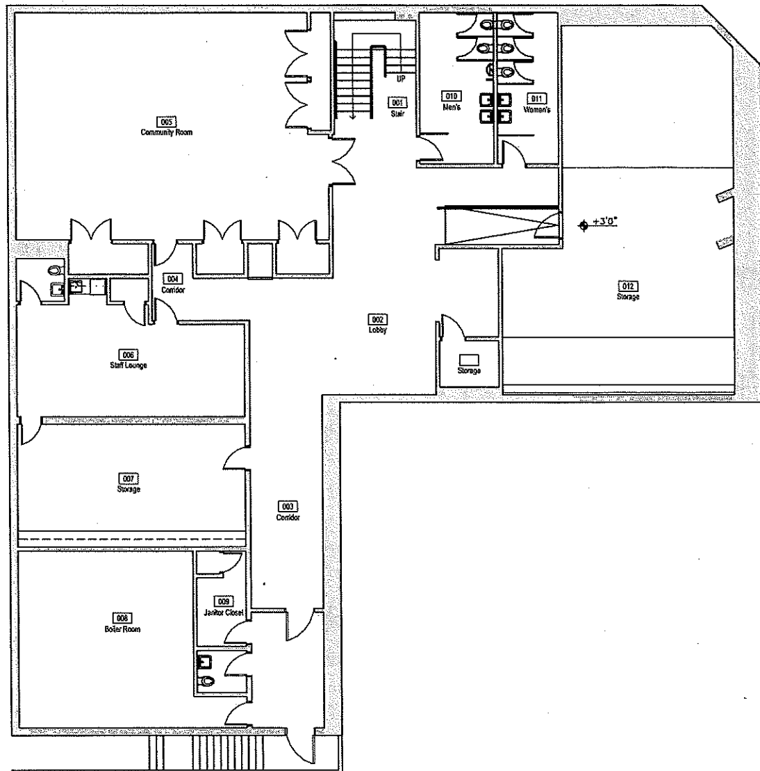
1 LOWER LEVEL PLAN 1/8" = 1'-0"
