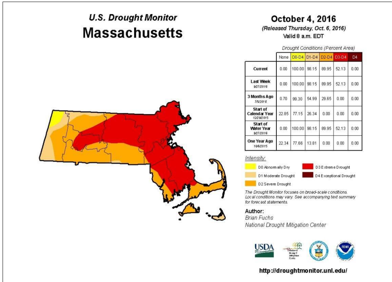
Source: US Drought Monitor, National Drought Mitigation Center
