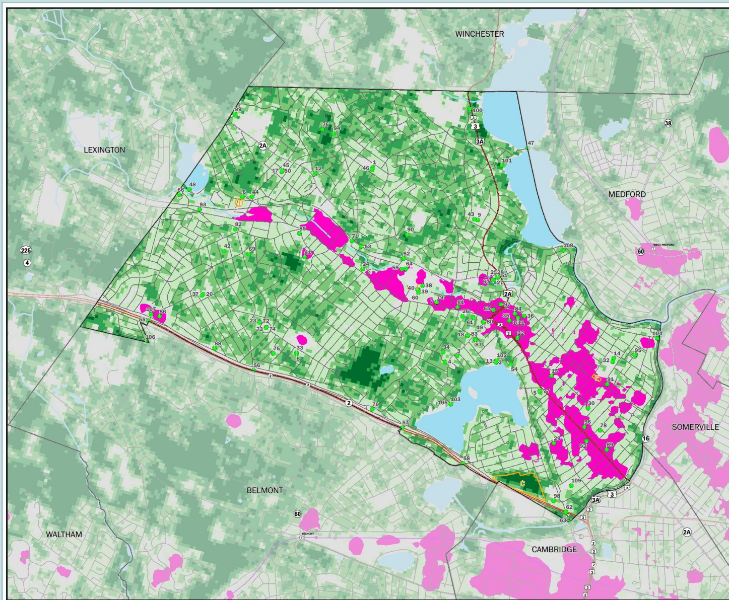
Map 10: High Land Surface Temperature
