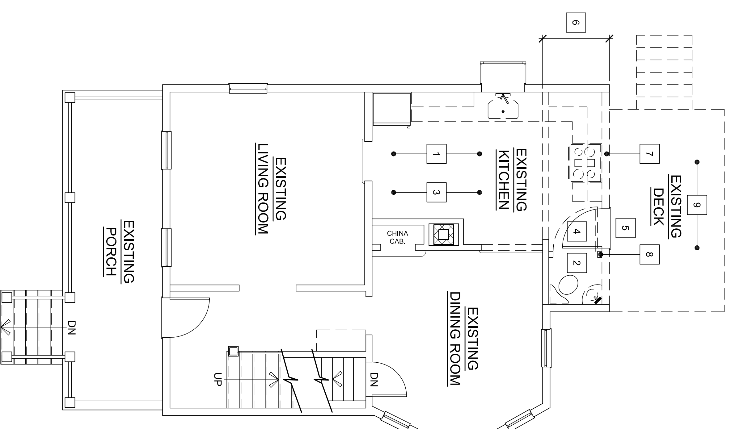
FIRST FLOOR EXISTING CONDITIONS / DEMOLITION PLAN SCALE: 1/4" = 1'-0"
