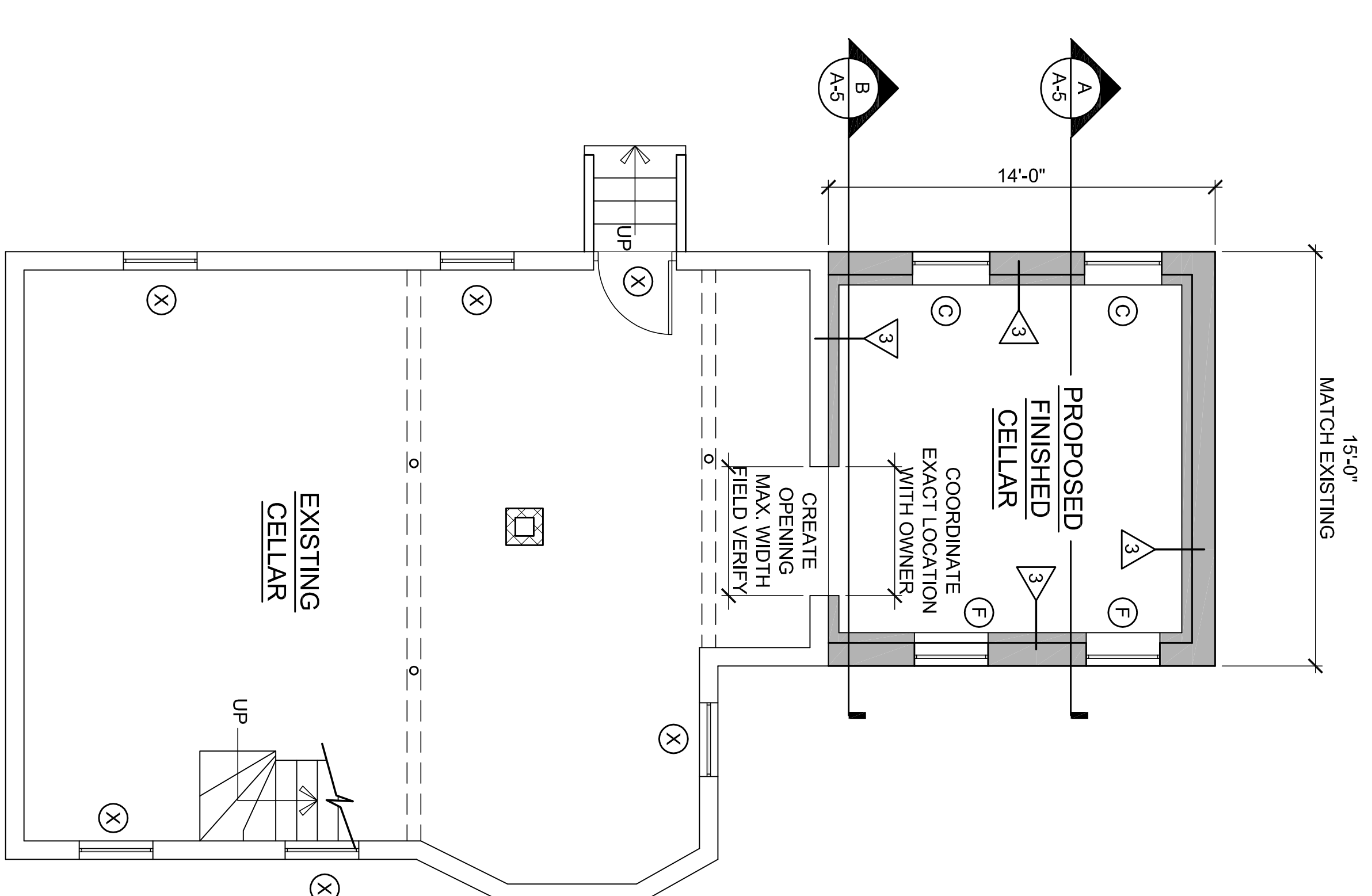
CELLAR CONSTRUCTION PLAN SCALE: 1/4" = 1'-0"
