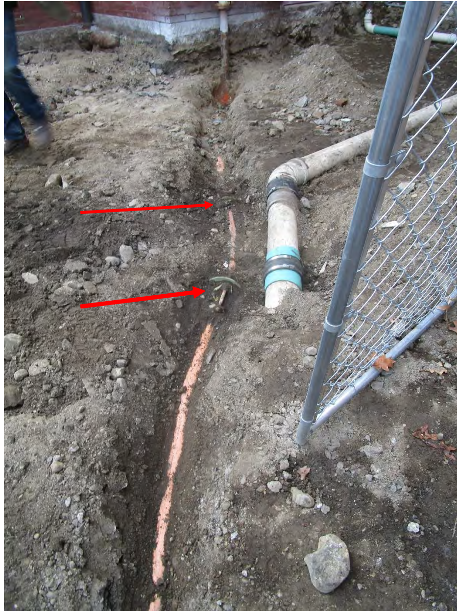
Existing gas service piping shallow depth and with 2 repair couplings
