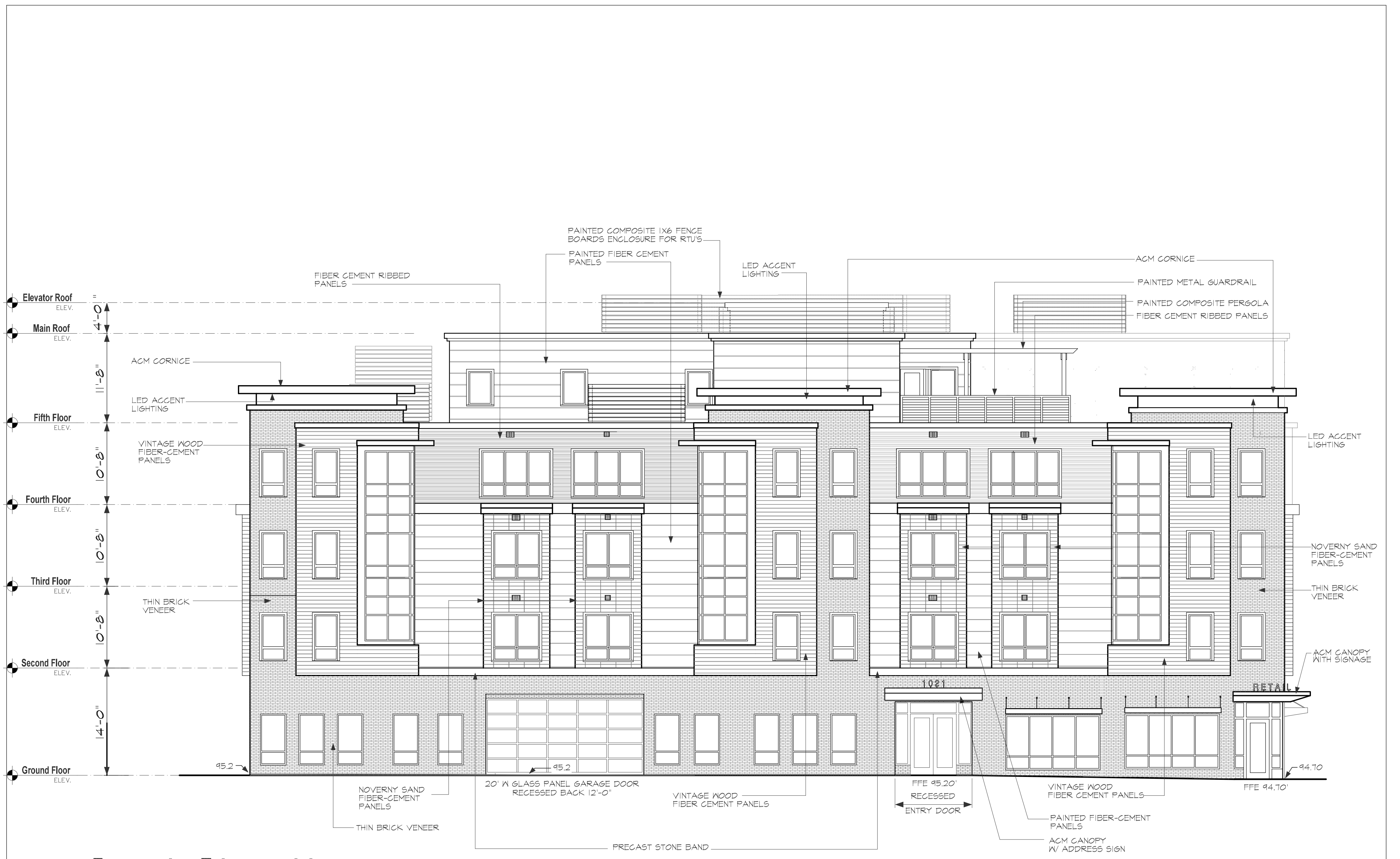
Front Elevation
