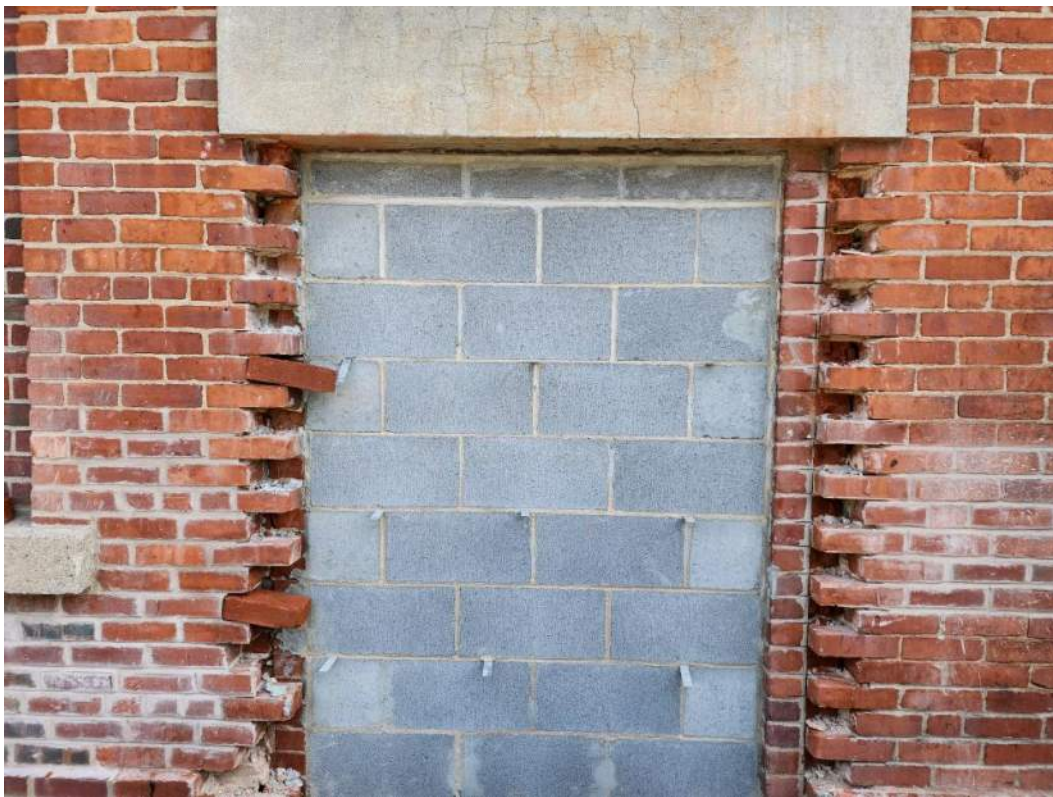
Photo #6 – Building D Masonry Infill in Progress (8/22/23)
