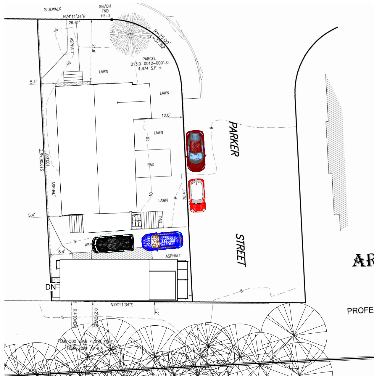
1 Site Plan 1" = 20'-0"
