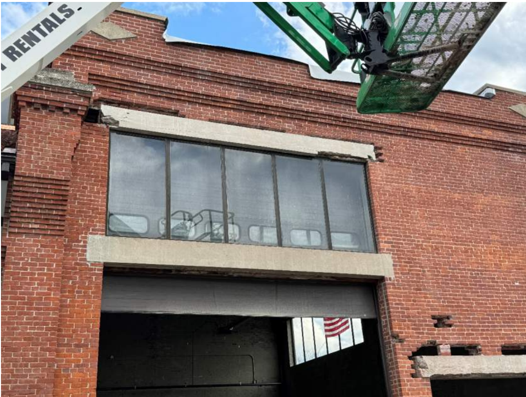
Photo #8 – Building D Lintel Replacement (10/17/23)
