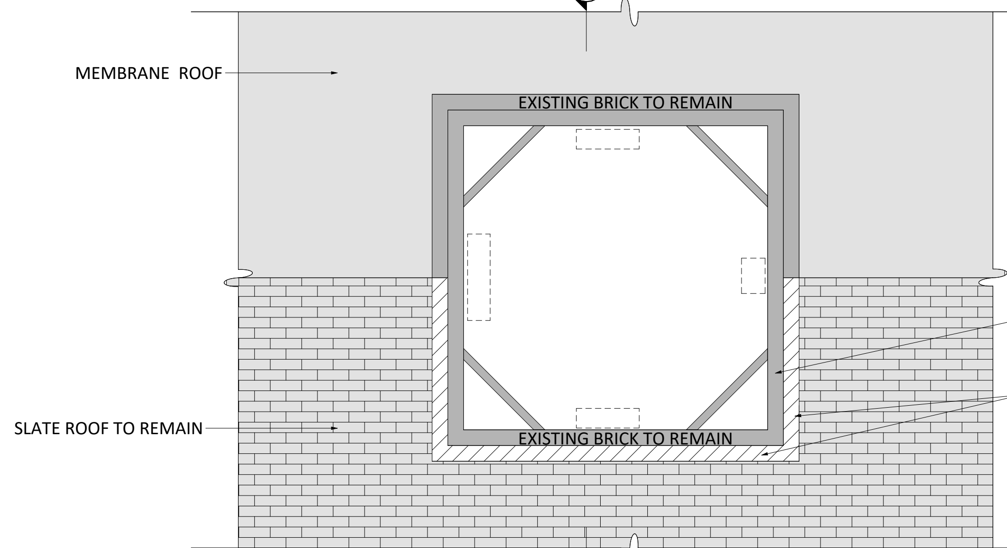
4 PART PLAN C 1/2" = 1'-0"
