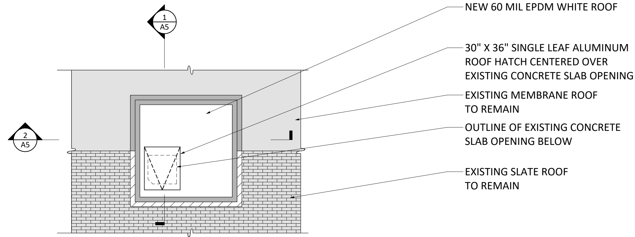
3 NEW ROOF PLAN 1/4" = 1'-0"
