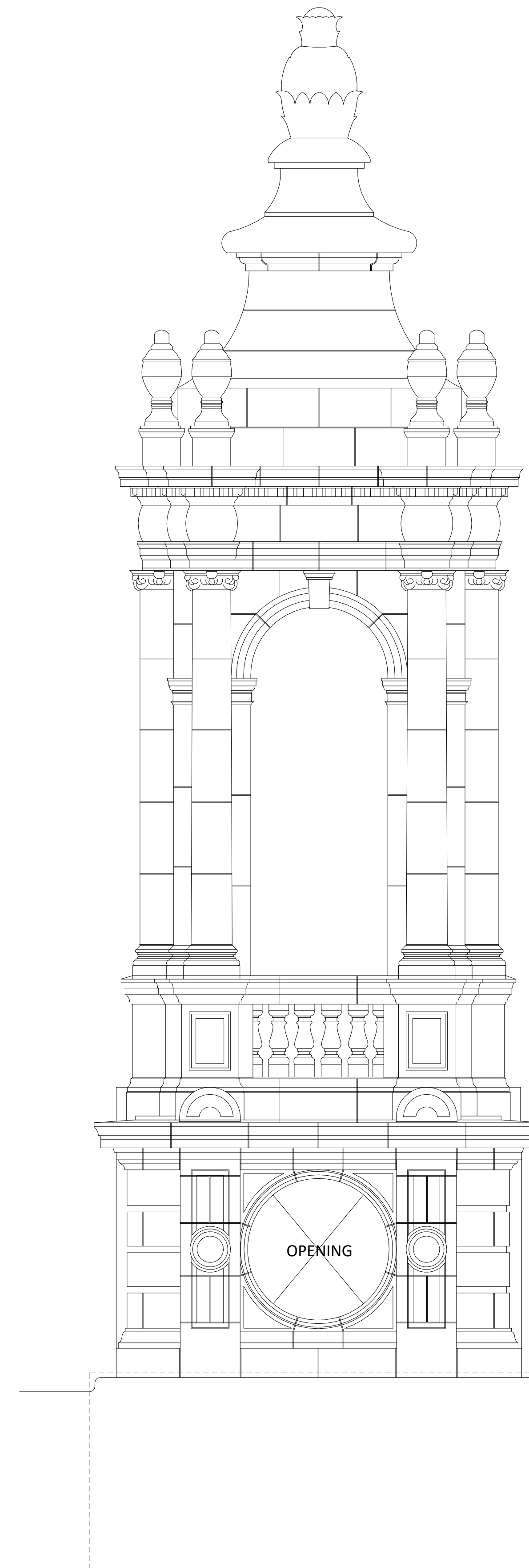
2 SOUTH ELEVATION 1/2" = 1'-0"
