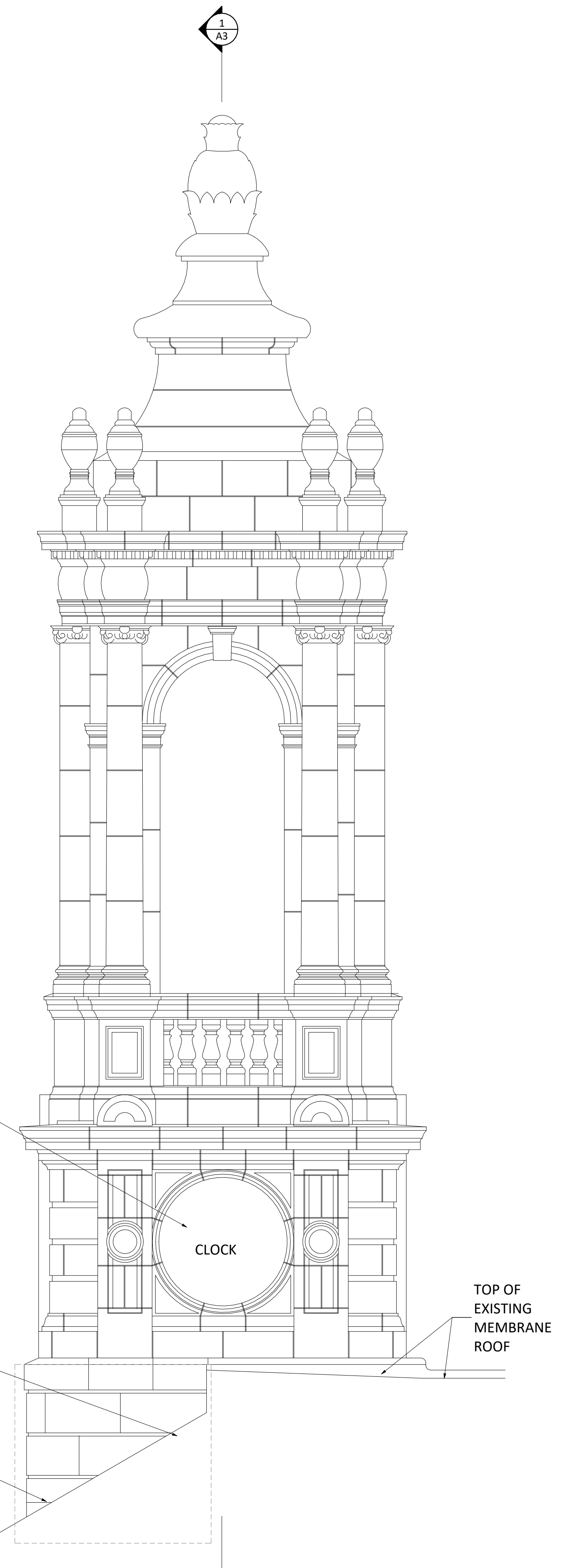
1 WEST ELEVATION 1/2" = 1'-0"
