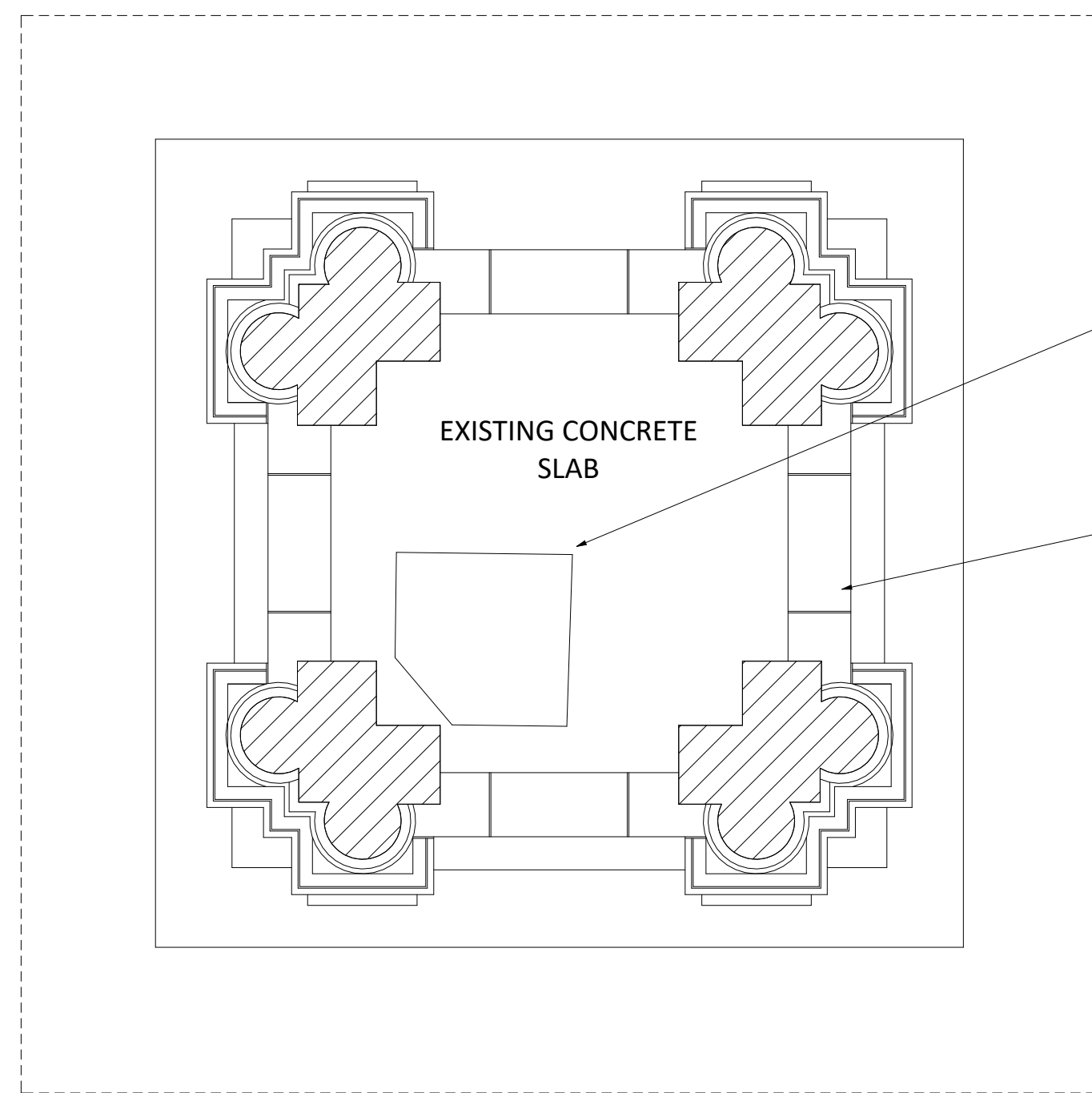
2 PART PLAN A 1/2" = 1'-0"
