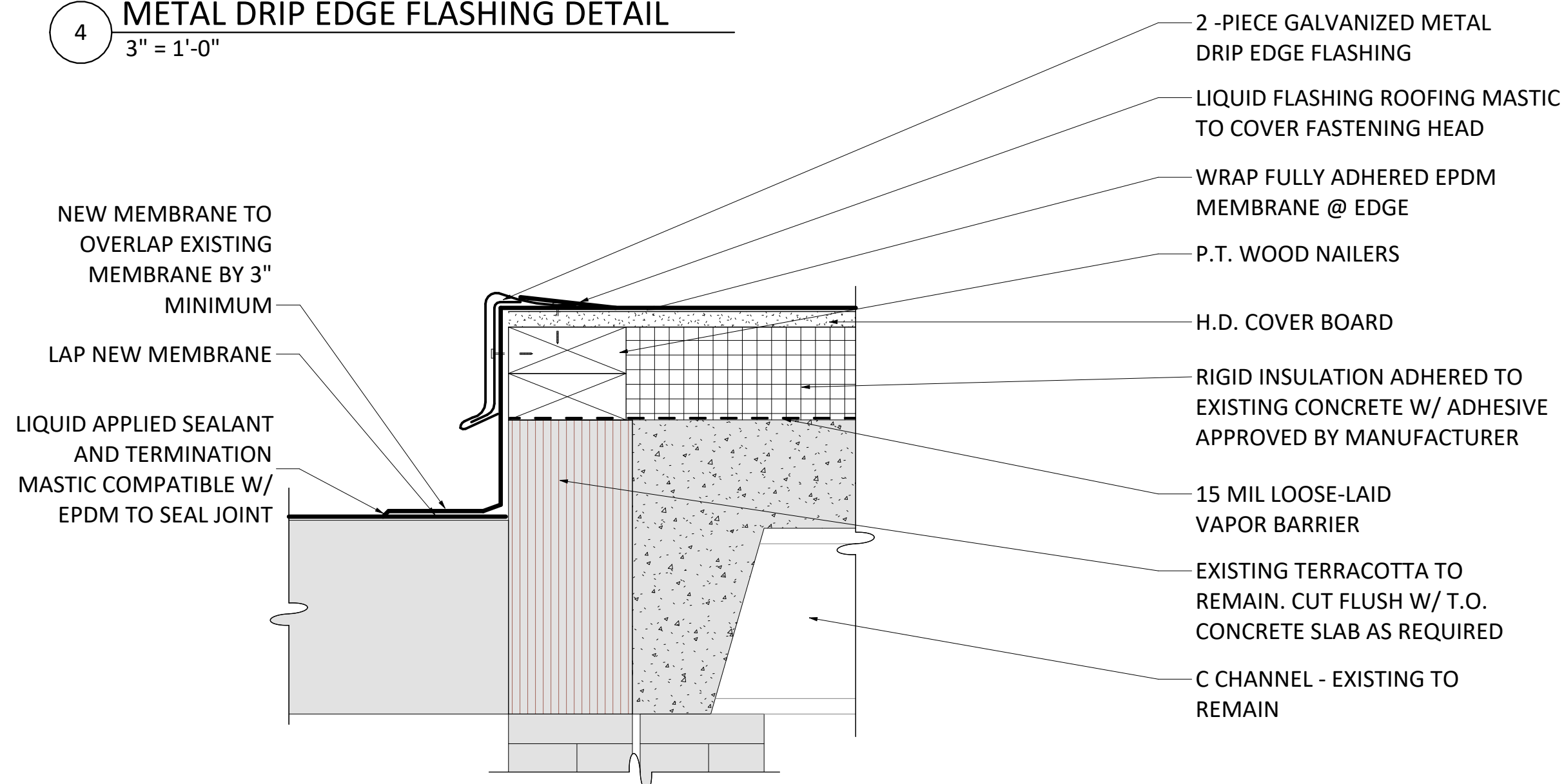
5 FLASHING @ FLAT ROOF 3" = 1'-0"
