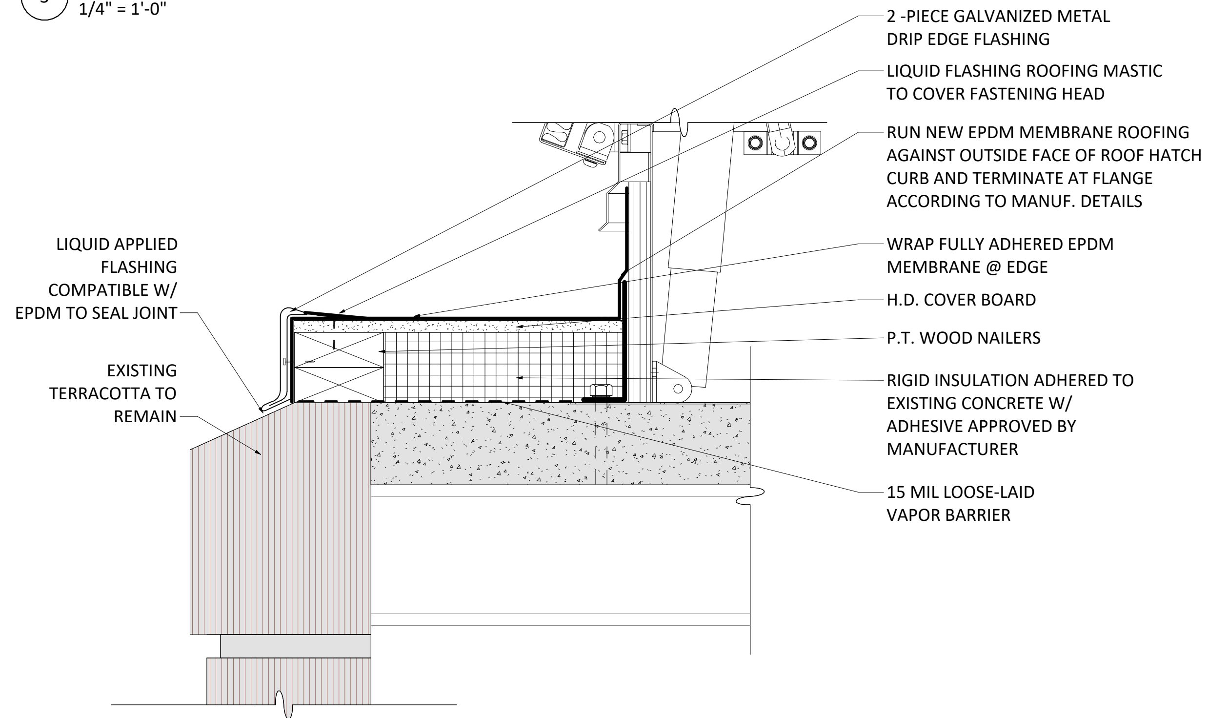
4 METAL DRIP EDGE FLASHING DETAIL 3" = 1'-0"
