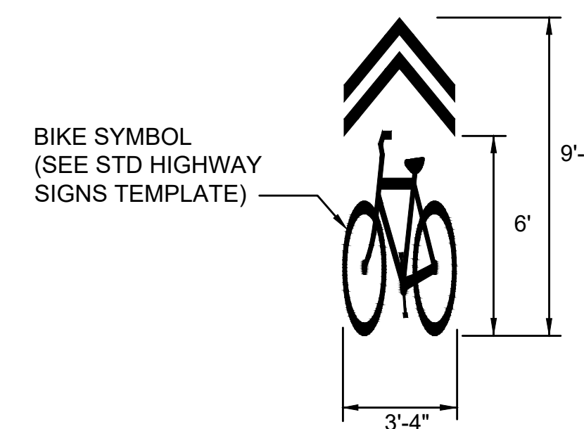
SHARED LANE MARKING NOT TO SCALE
