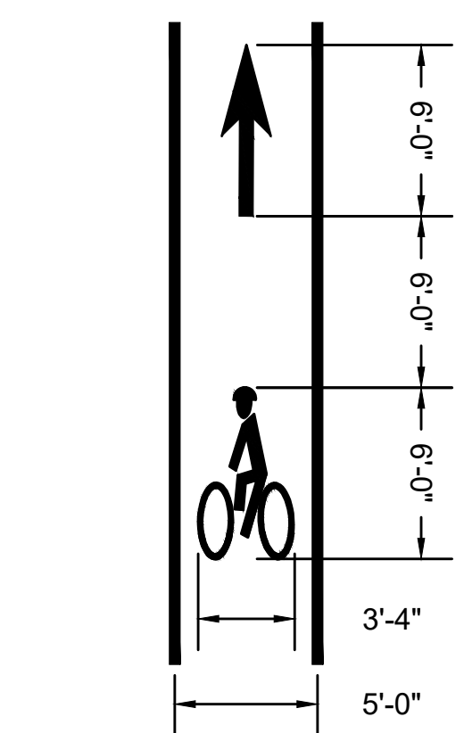
BIKE LANE MARKING NOT TO SCALE
