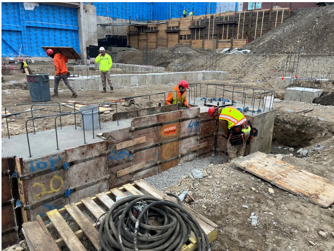
Photograph 2: Concrete grade beams & pile caps.
