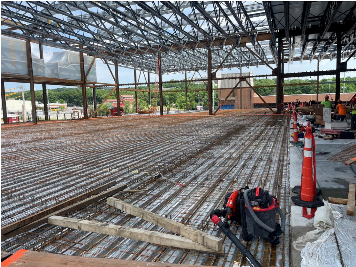
Photograph 2: Level 2 rebar install.
